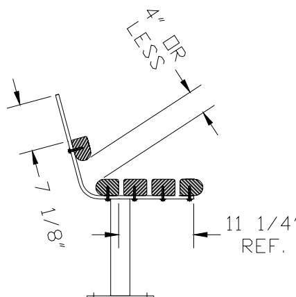
Diagram 3: Bench 4-foot length 140401 shown (attaching back boards)
