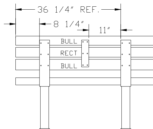
Diagram 3: Bench 4-foot length 140401 shown (attaching back boards)
