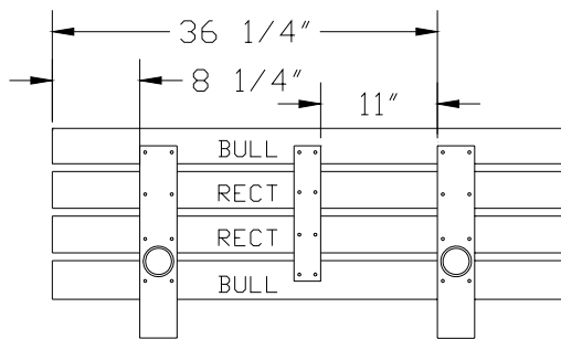
Diagram 2: Bench 4-foot length 140401 shown (attaching seat boards)
