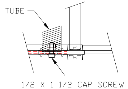
Detail A: Attaching end castings and fastening tubes
